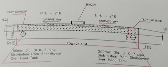
TYPICAL C-SECTION 1-1
