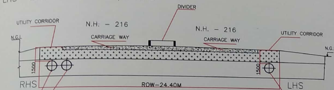
TYPICAL C-SECTION 2-2
